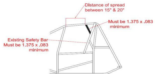
#2 Support Bar
