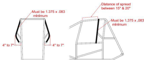
#1 Support Bar
